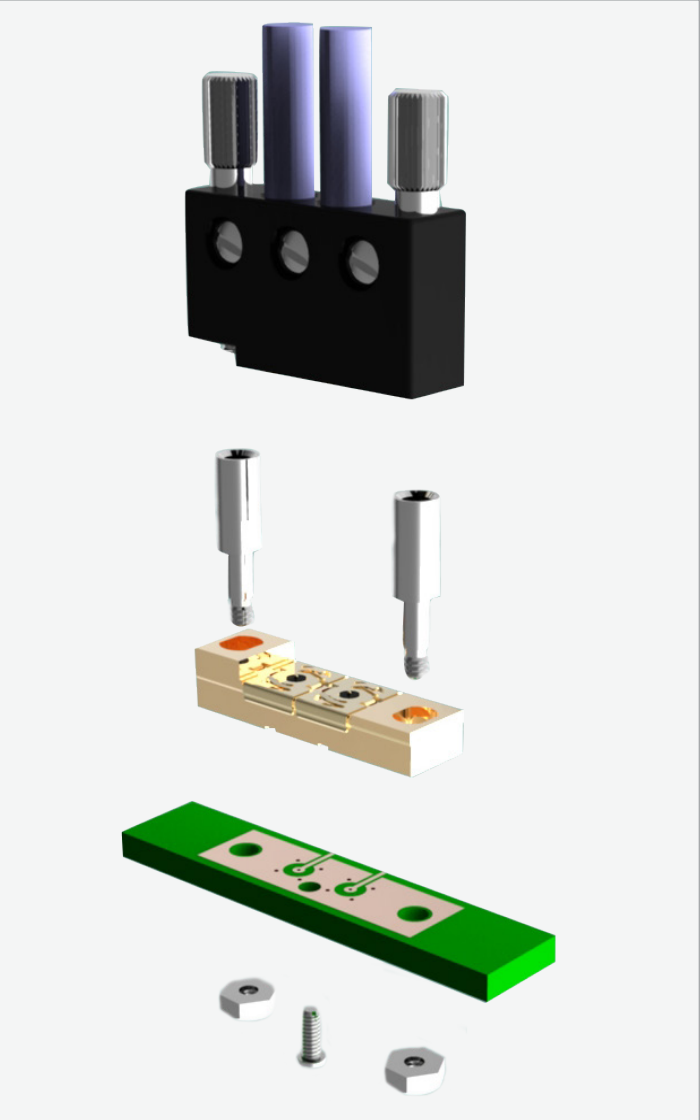
Vertical Mount
